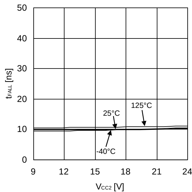
Figure 42. Fall time
