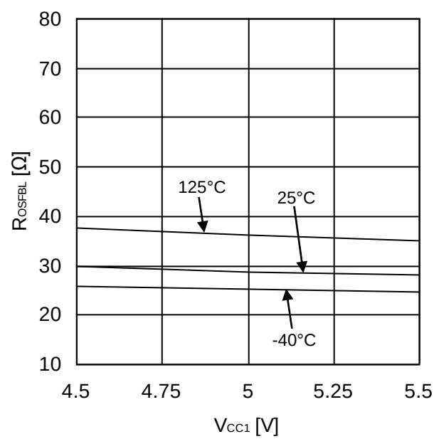
Figure 76. OSFB Output ON-Resistance ( I_{OSFB}=5mA )
