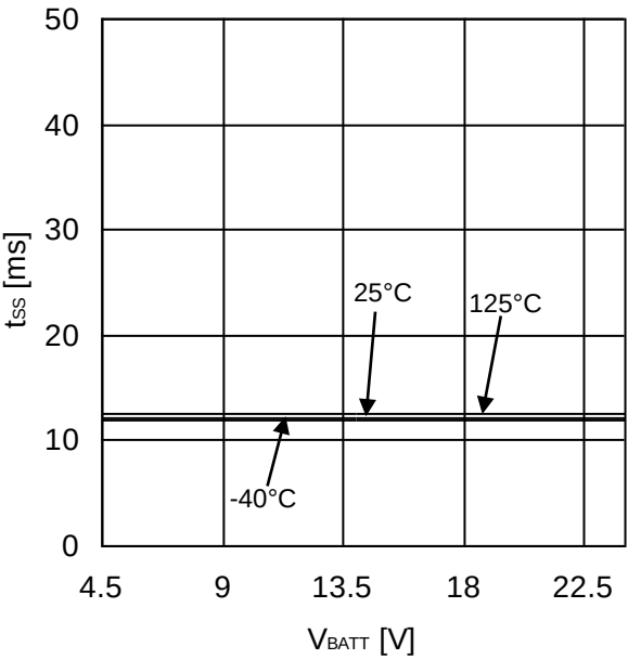
Figure 24. Soft-start Time
