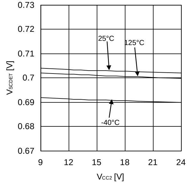
Figure 66. Short Current Detection Voltage
