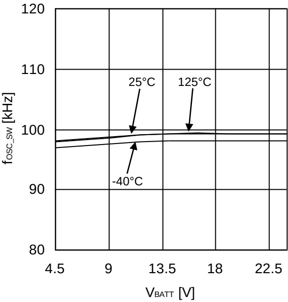
Figure 23. Oscillation Frequency
