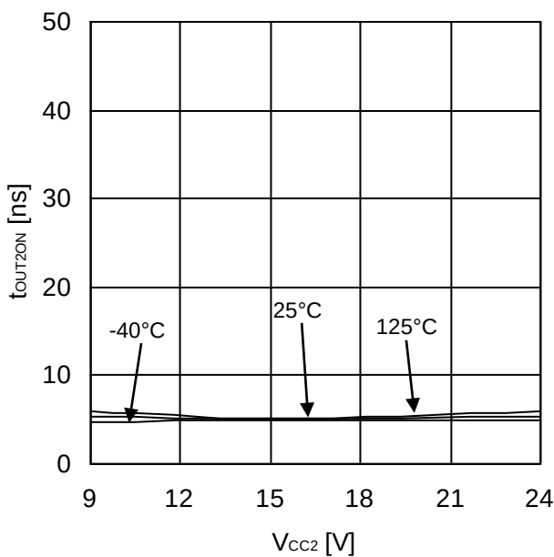
Figure 46. OUT2 Output Delay Time
