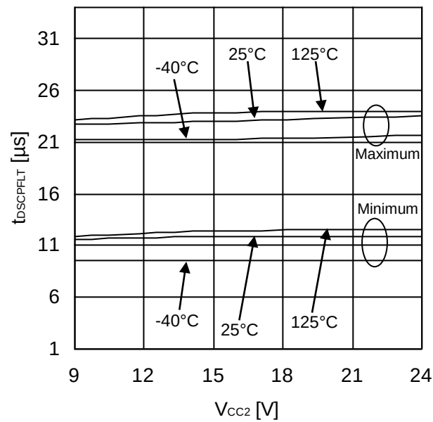
Figure 70. Short Current Detection Delay time (FLT)
