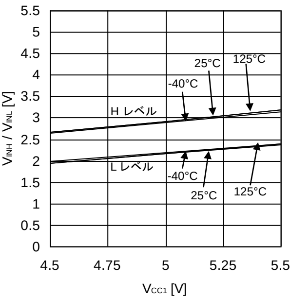
Figure 31. Logic High / Low Level Input Voltage (INA, DIS)
