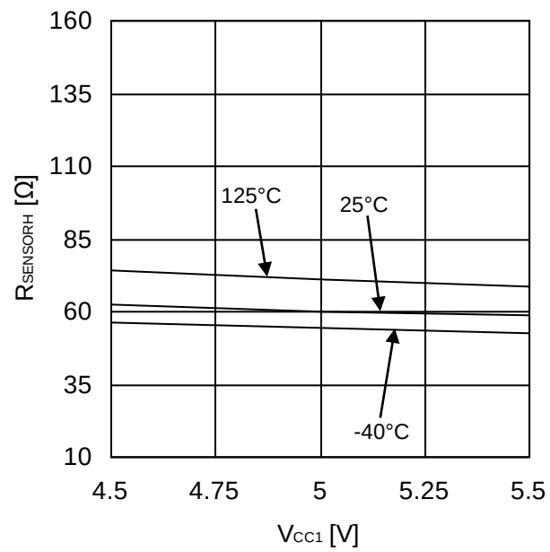
Figure 56. SENSOR ON Resistance(Source-side) (I SEN =5mA)
