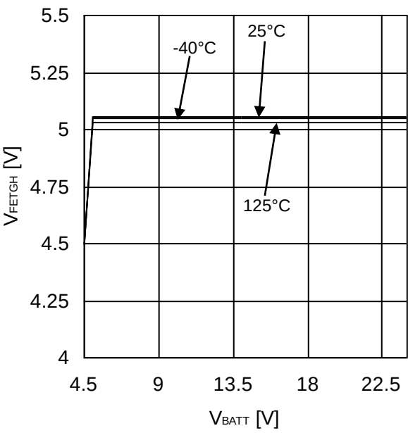
Figure 19. FET_G Output Voltage H1/H2
