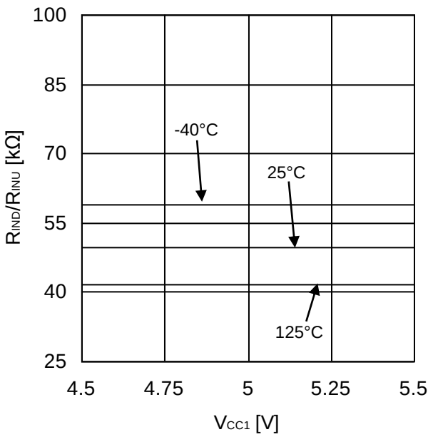
Figure 32. Logic Pull-Down Resistance (INA) Pull-Up Resistance (DIS)
