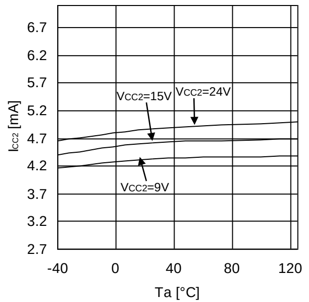
Figure 16. Output Side Circuit Current (OUT=L, R TC =10kΩ)
