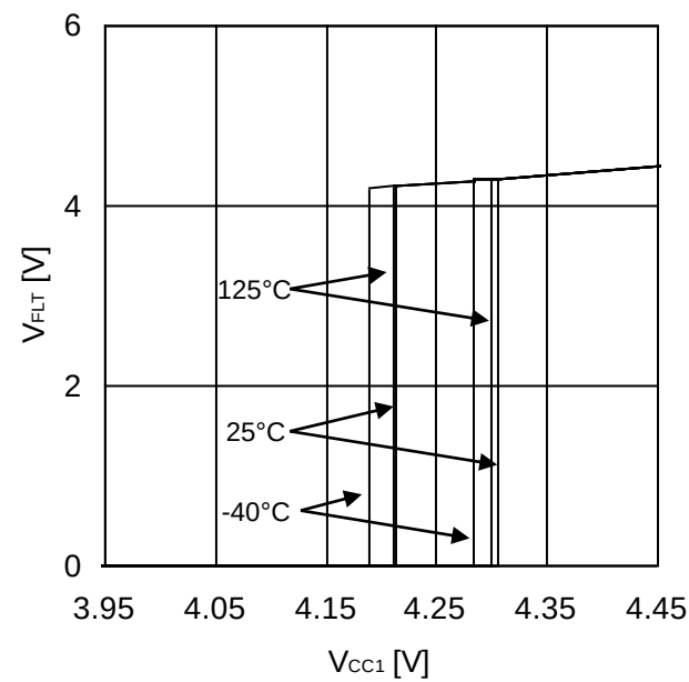
Figure 58. Input-side UVLO ON/OFF Voltage
