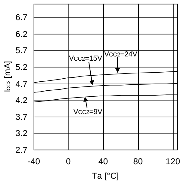
Figure 18. Output Side Circuit Current (OUT=H, R TC =10kΩ)
