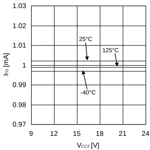
Figure 48. TOx Pin Output Current (RTC=10kΩ)
