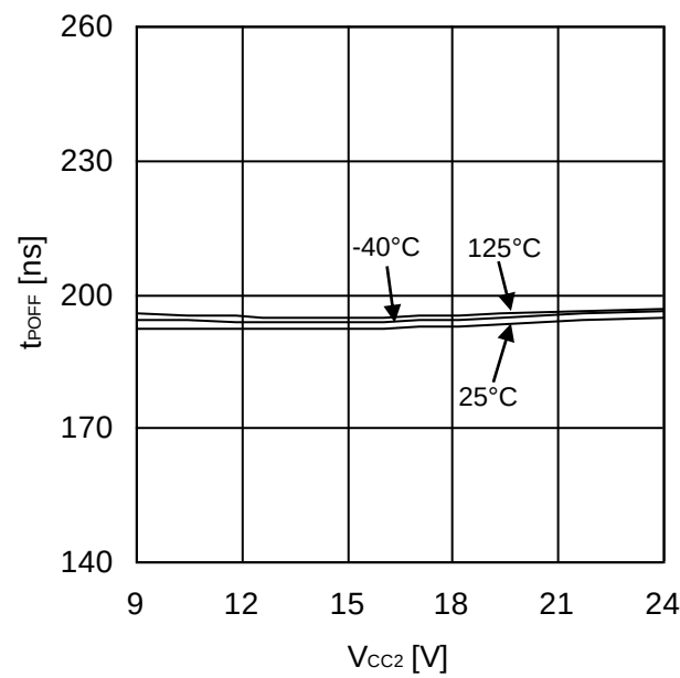
Figure 40. Turn OFF time
