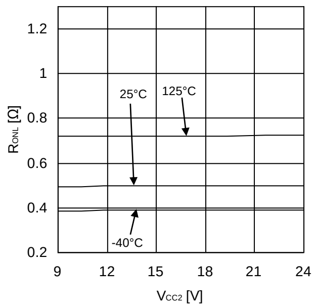
Figure 38. OUT1 ON-Resistance (Sink-side) ( I_{OUT1}=40mA )
