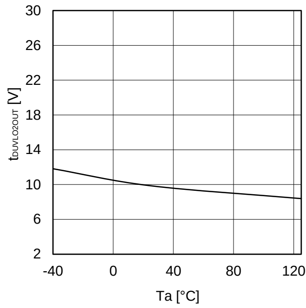
Figure 64. Output-side UVLO Delay Time (OUT1)
