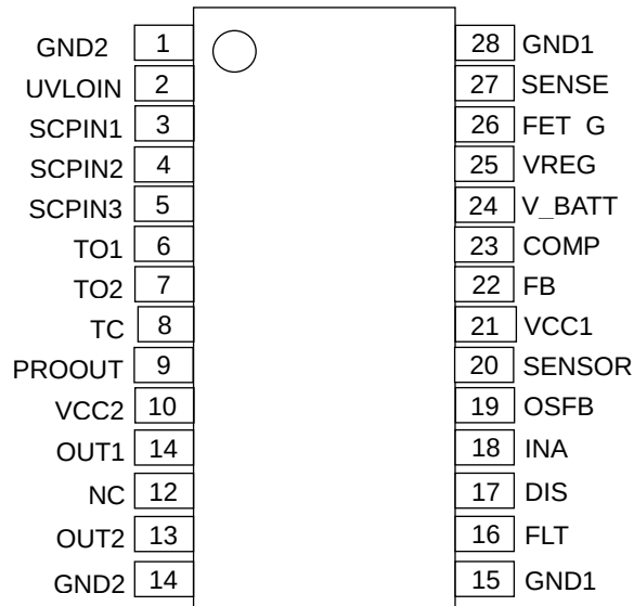
Figure 2. Pin configuration
