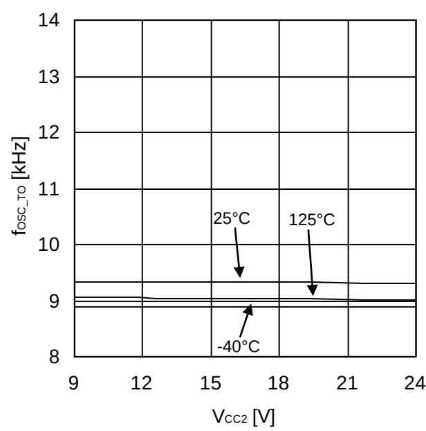
Figure 50. SENSOR Output Frequency
