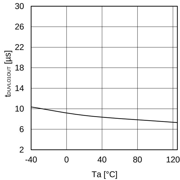
Figure 60. Input-side UVLO Delay Time (OUT1)
