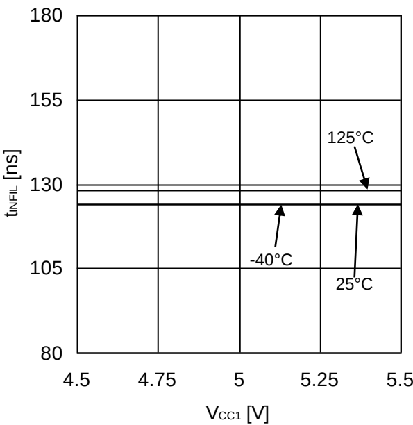
Figure 33. Logic Input Filtering Time (L pulse)
