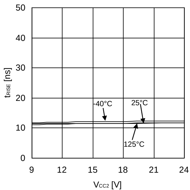
Figure 41. Rise time
