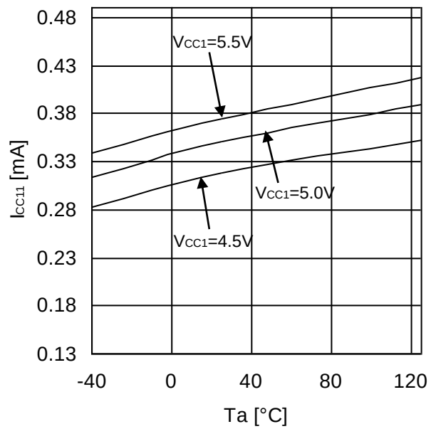
Figure 8. Input Side Circuit Current 1 (OUT1=L)
