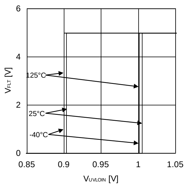
Figure 62. Output-side UVLO ON / OFF Threshold Voltage
