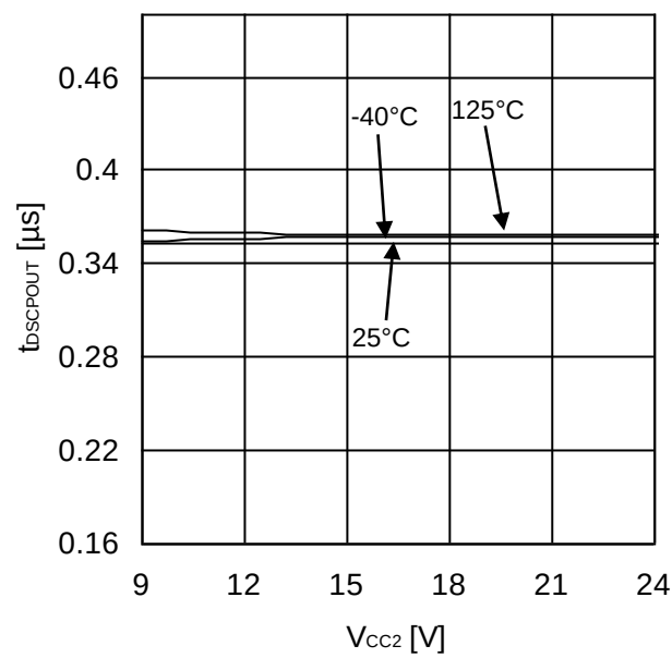
Figure 68. Short Current Detection Delay time (OUT1)
