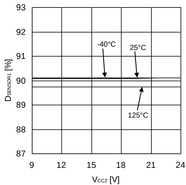
Figure 52. SENSOR Output Duty1 (V TOx =1.35V)
