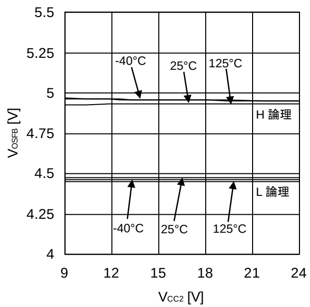
Figure 74. Gate State H/L Detection Threshold Voltage
