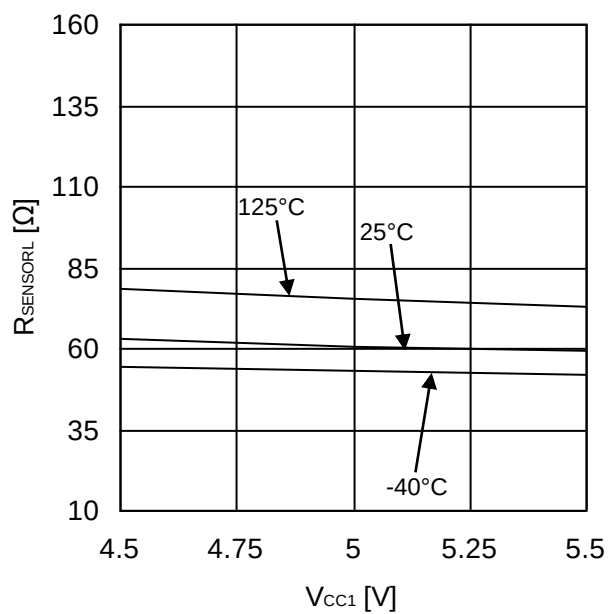
Figure 57. SENSOR ON Resistance (Sink-side) (I SEN =5mA)
