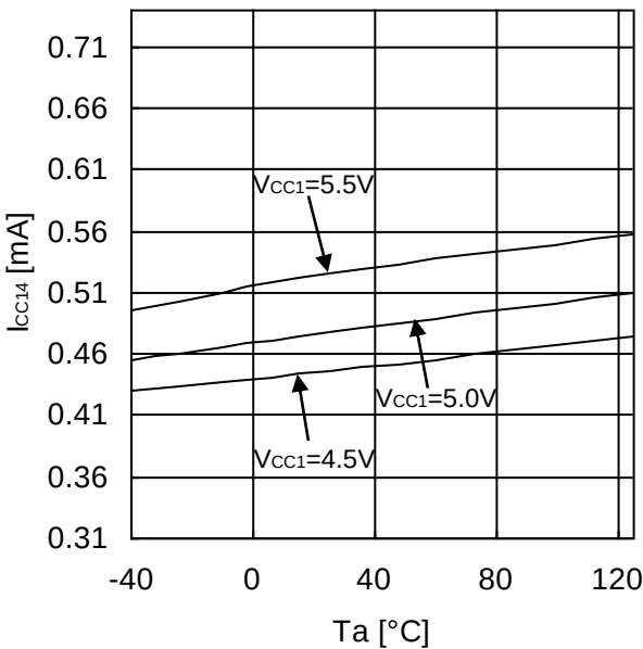
Figure 14. Input Side Circuit Current 4 (INA=20kHz, Duty=50%)
