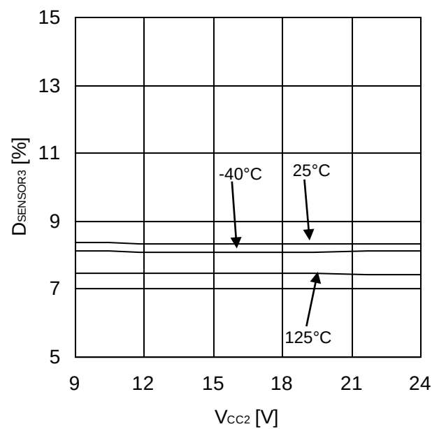
Figure 54. SENSOR Output Duty3 (V TOx =3.84V)
