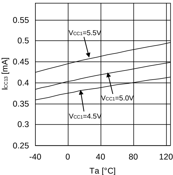
Figure 12. Input Side Circuit Current 3 (INA=10kHz, Duty=50%)
