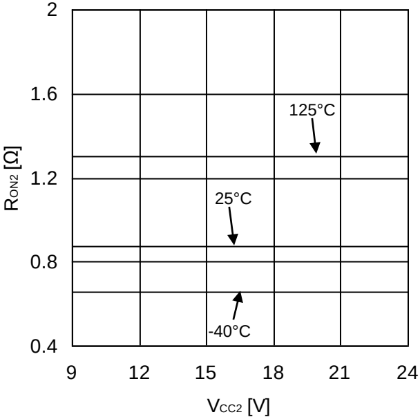
Figure 44. OUT2 ON-Resistance (I OUT2 =40mA)
